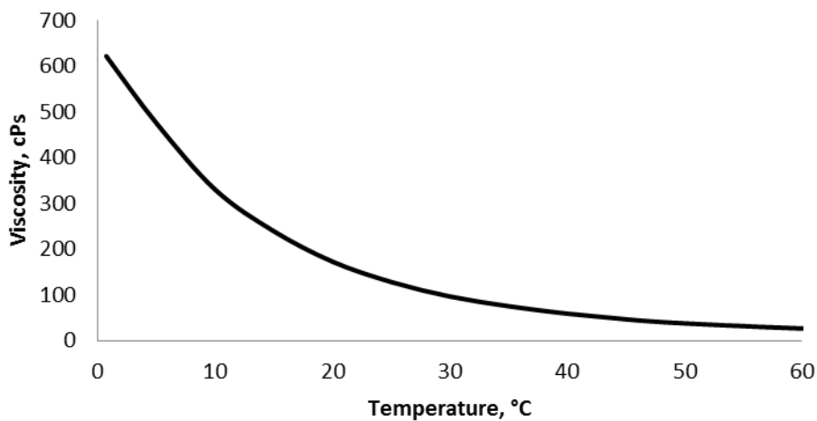
Viscosity as a Function of Temperature
