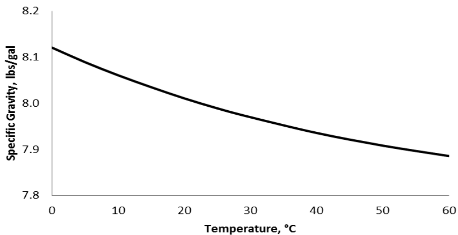
Specific Gravity as a Function of Temperature
